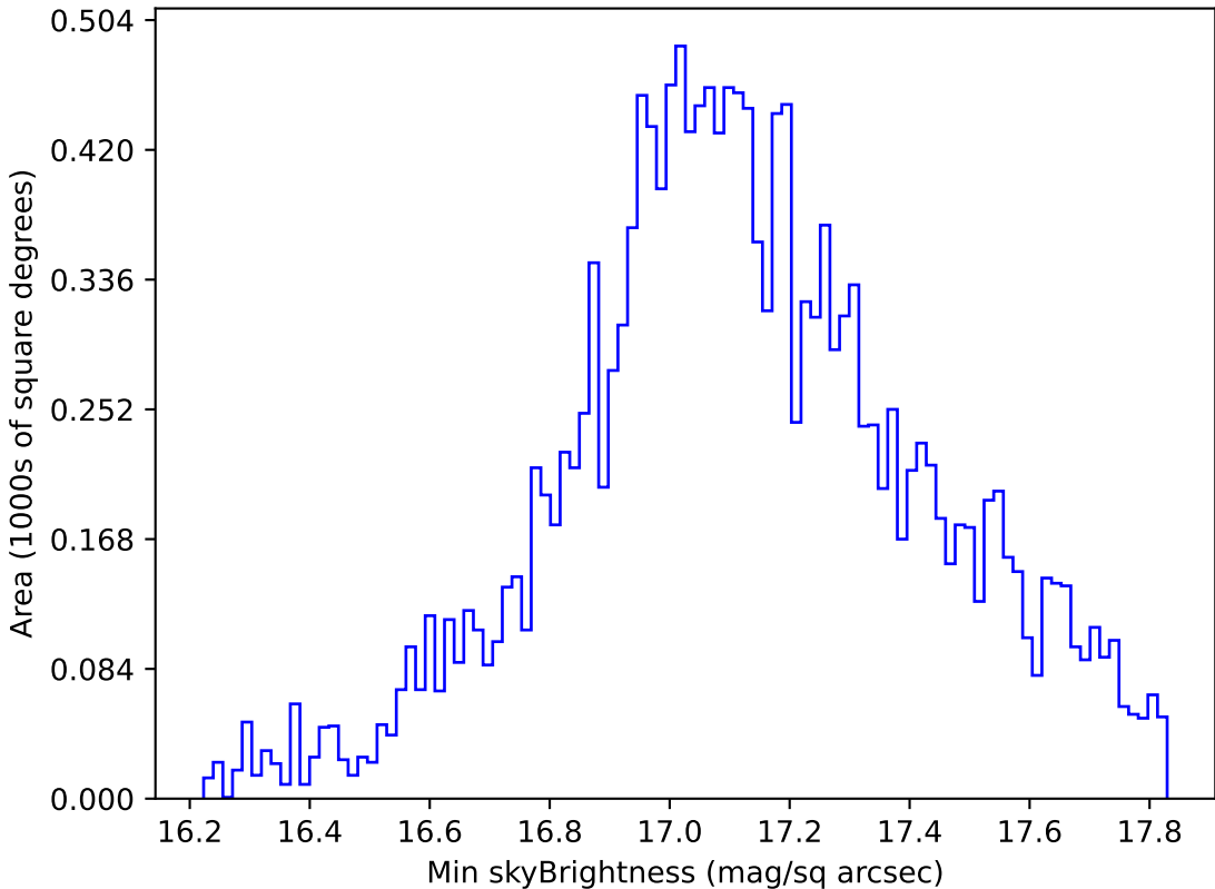
roll_pause_mjdp0_v3.4_10yrs WFD y band: Min skyBrightness
