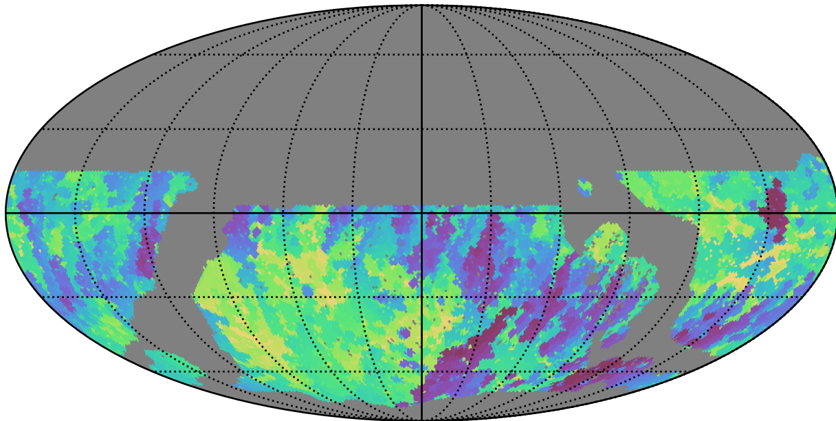
roll_pause_mjdp0_v3.4_10yrs WFD r band: Min skyBrightness
