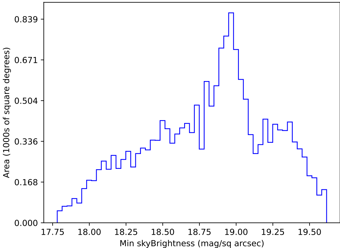
roll_pause_mjdp0_v3.4_10yrs WFD r band: Min skyBrightness
