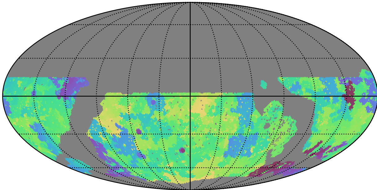
roll_pause_mjdp0_v3.4_10yrs WFD g band: Min skyBrightness
