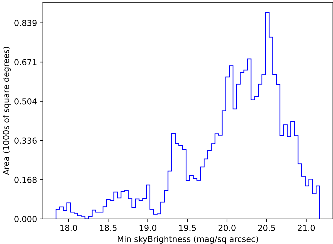
roll_pause_mjdp0_v3.4_10yrs WFD g band: Min skyBrightness
