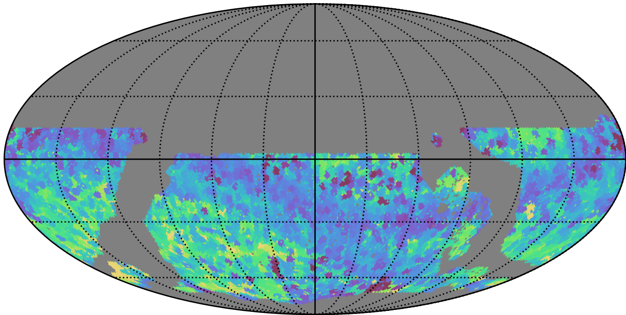
roll_pause_mjdp0_v3.4_10yrs WFD all bands: Min skyBrightness
