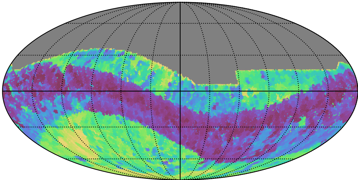
roll_pause_mjdp0_v3.4_10yrs All sky z band: Min skyBrightness
