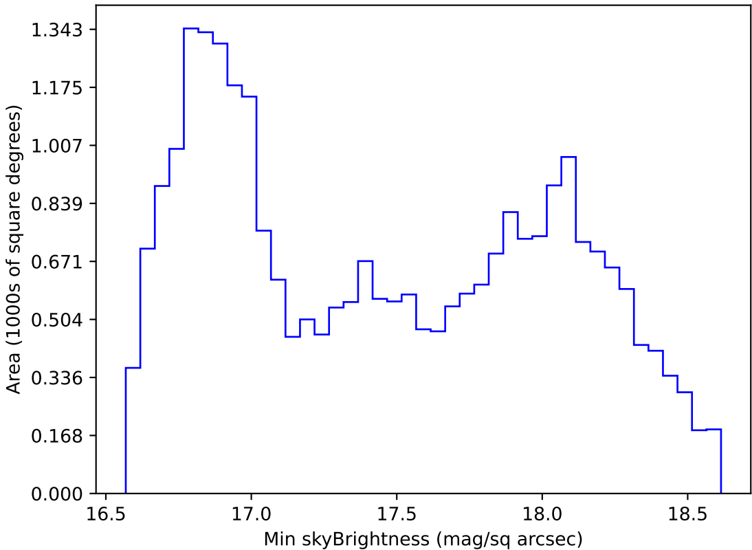
roll_pause_mjdp0_v3.4_10yrs All sky z band: Min skyBrightness
