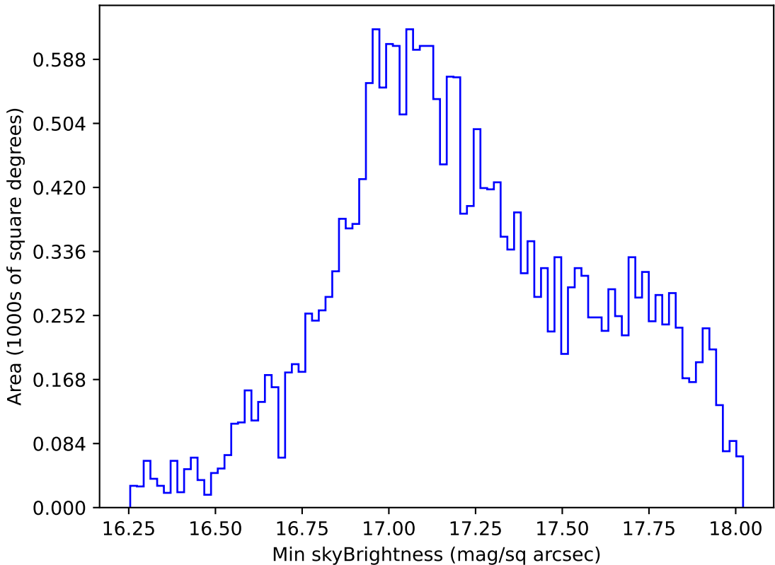
roll_pause_mjdp0_v3.4_10yrs All sky y band: Min skyBrightness
