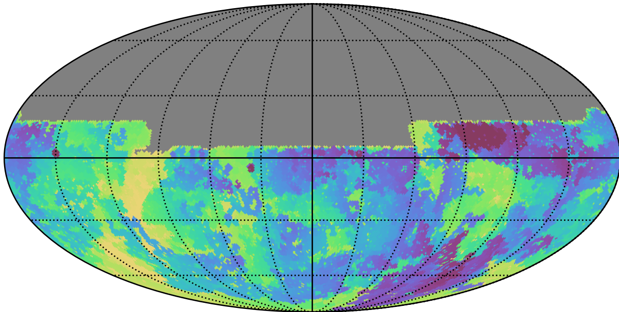
roll_pause_mjdp0_v3.4_10yrs All sky u band: Min skyBrightness
