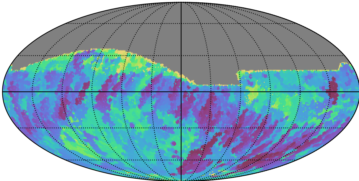
roll_pause_mjdp0_v3.4_10yrs All sky r band: Min skyBrightness
