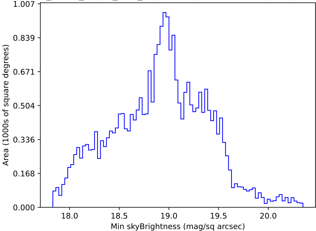
roll_pause_mjdp0_v3.4_10yrs All sky r band: Min skyBrightness
