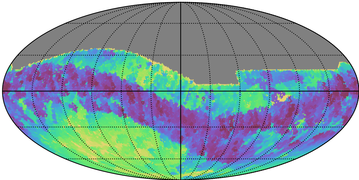
roll_pause_mjdp0_v3.4_10yrs All sky i band: Min skyBrightness
