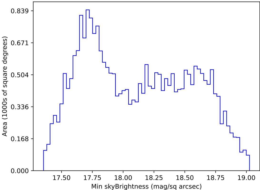
roll_pause_mjdp0_v3.4_10yrs All sky i band: Min skyBrightness
