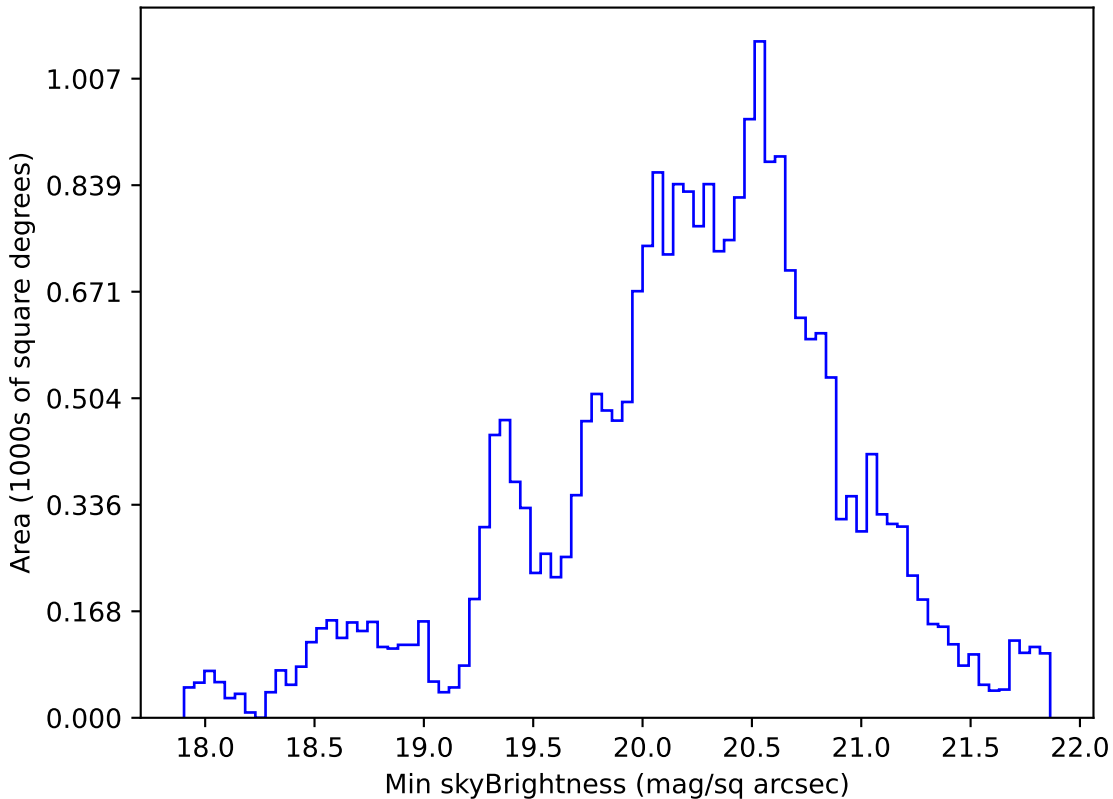
roll_pause_mjdp0_v3.4_10yrs All sky g band: Min skyBrightness
