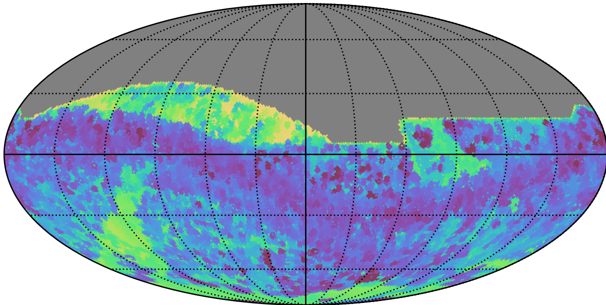
roll_pause_mjdp0_v3.4_10yrs All sky all bands: Min skyBrightness
