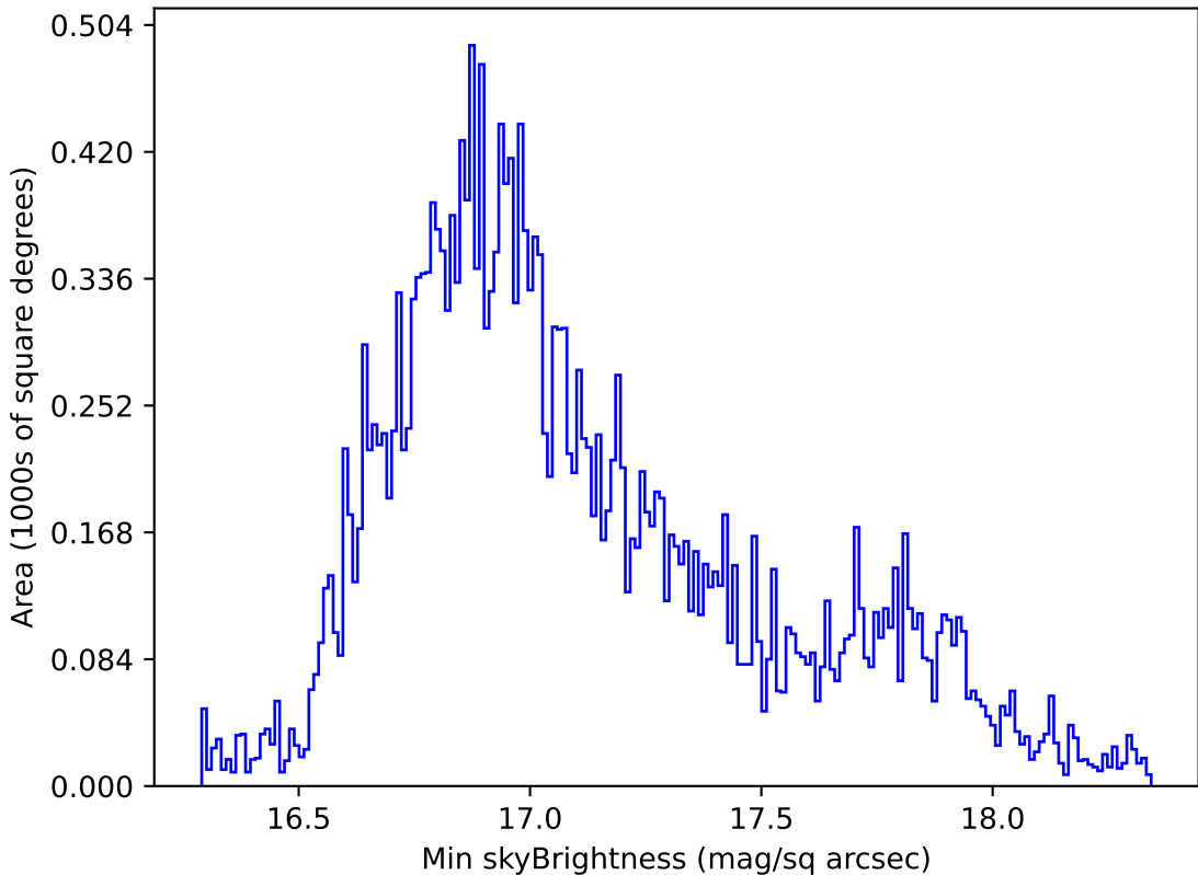
roll_pause_mjdp0_v3.4_10yrs All sky all bands: Min skyBrightness
