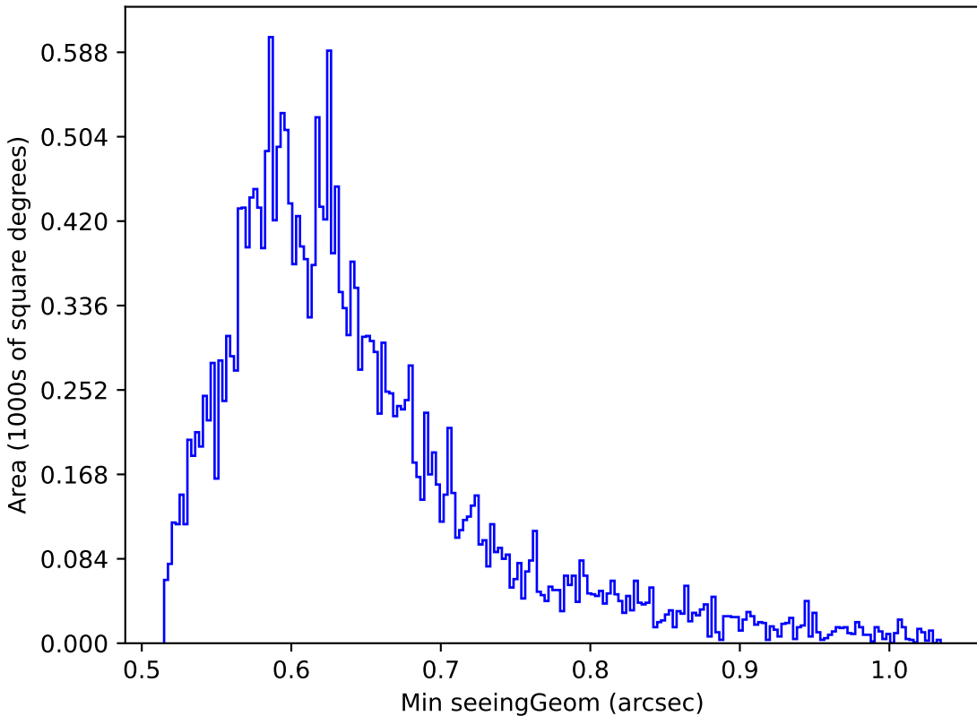
roll_pause_mjdp0_v3.4_10yrs Yr 1 z band: Min seeingGeom
