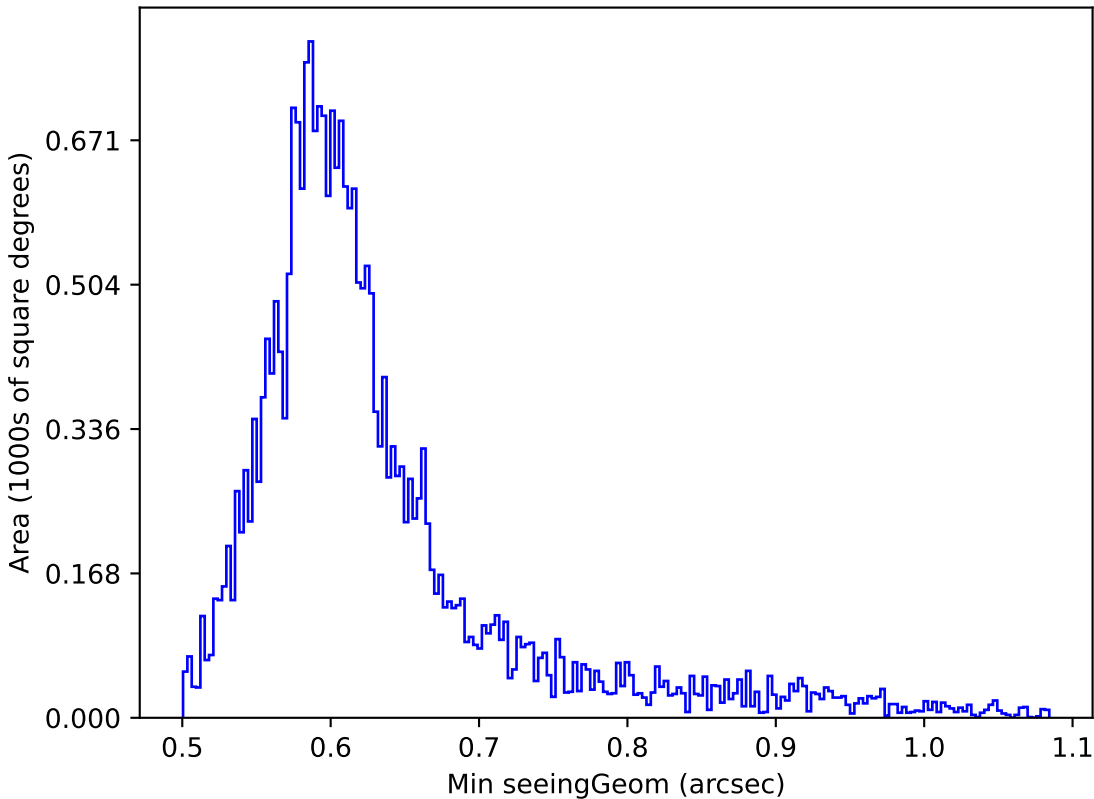
roll_pause_mjdp0_v3.4_10yrs Yr 1 i band: Min seeingGeom
