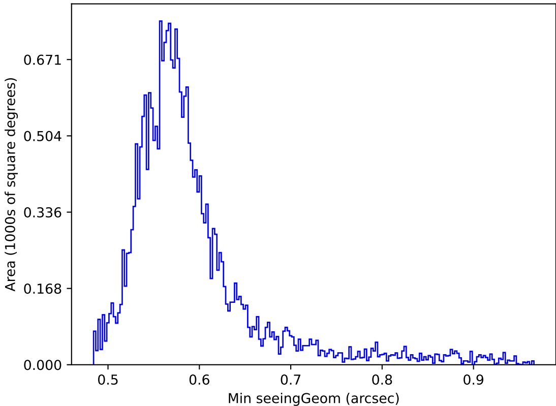
roll_pause_mjdp0_v3.4_10yrs Yr 1 all bands: Min seeingGeom
