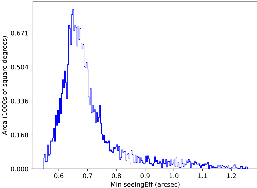
roll_pause_mjdp0_v3.4_10yrs Yr 1 i band: Min seeingEff
