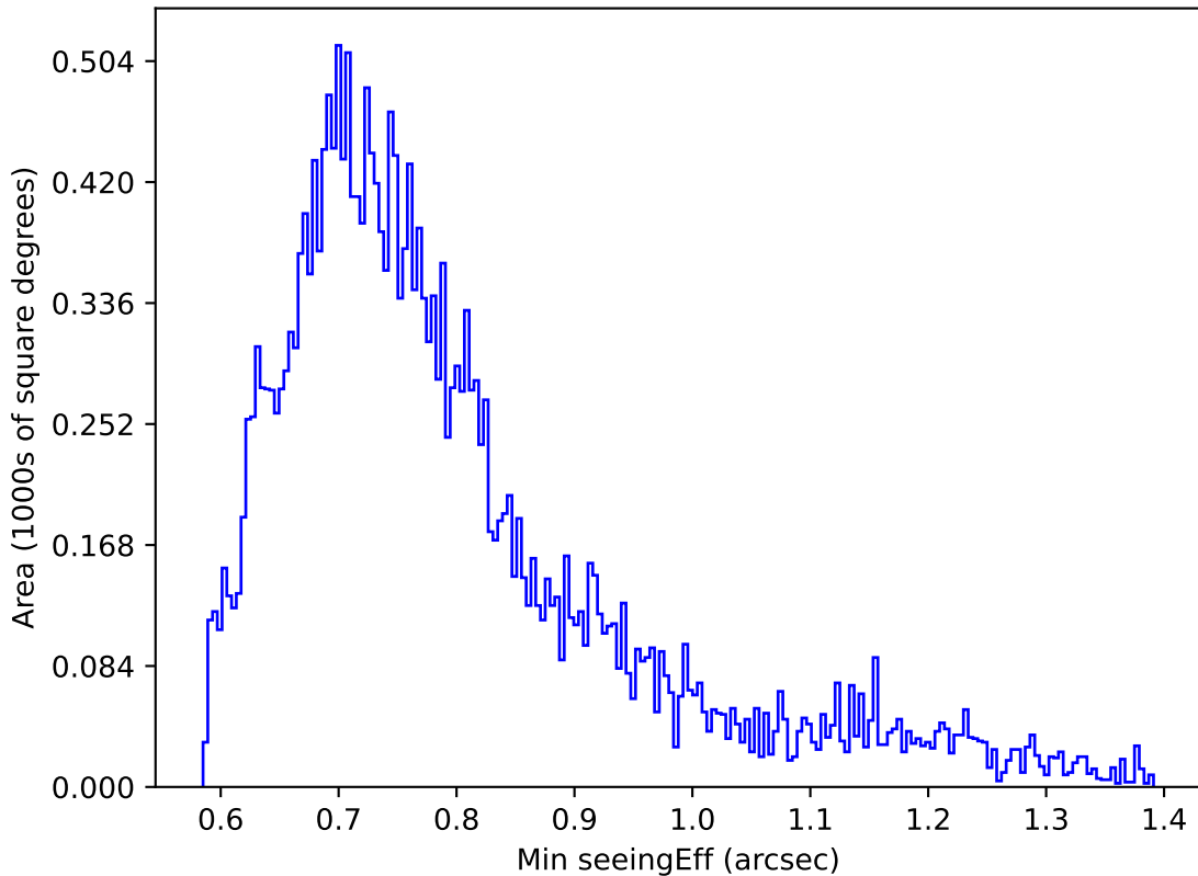
roll_pause_mjdp0_v3.4_10yrs Yr 1 g band: Min seeingEff
