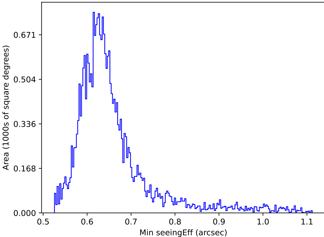
roll_pause_mjdp0_v3.4_10yrs Yr 1 all bands: Min seeingEff
