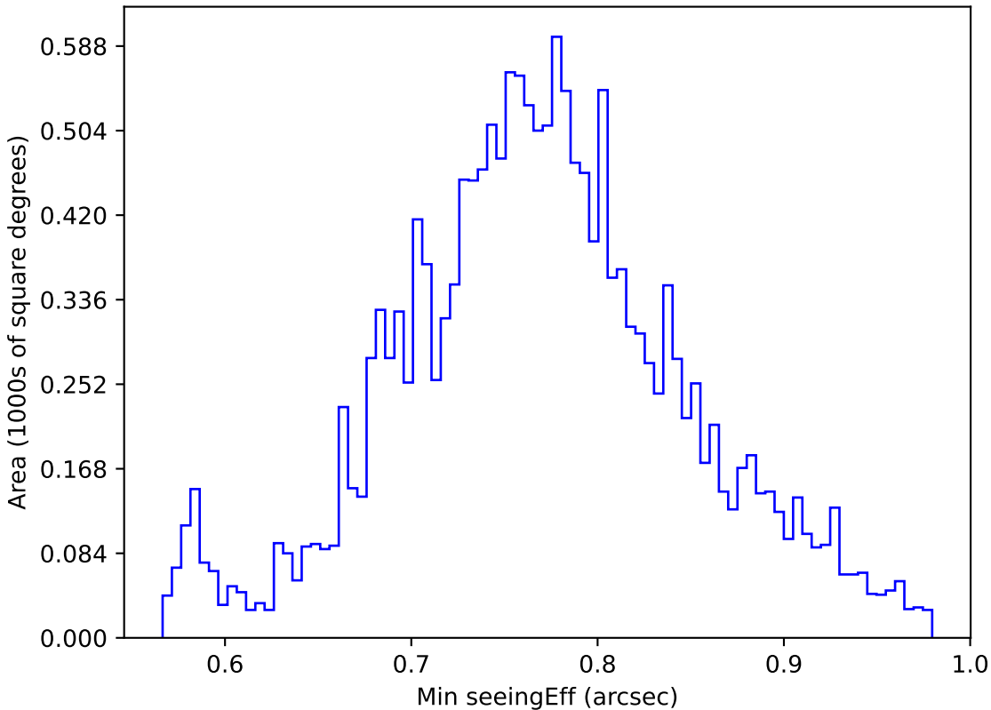
roll_pause_mjdp0_v3.4_10yrs WFD u band: Min seeingEff
