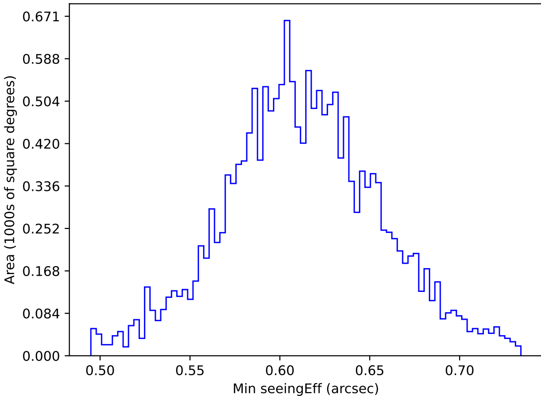
roll_pause_mjdp0_v3.4_10yrs WFD r band: Min seeingEff
