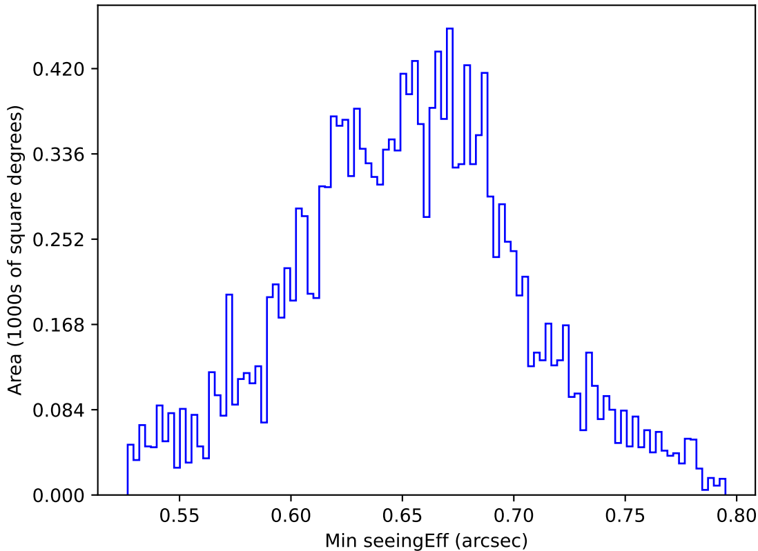
roll_pause_mjdp0_v3.4_10yrs WFD g band: Min seeingEff
