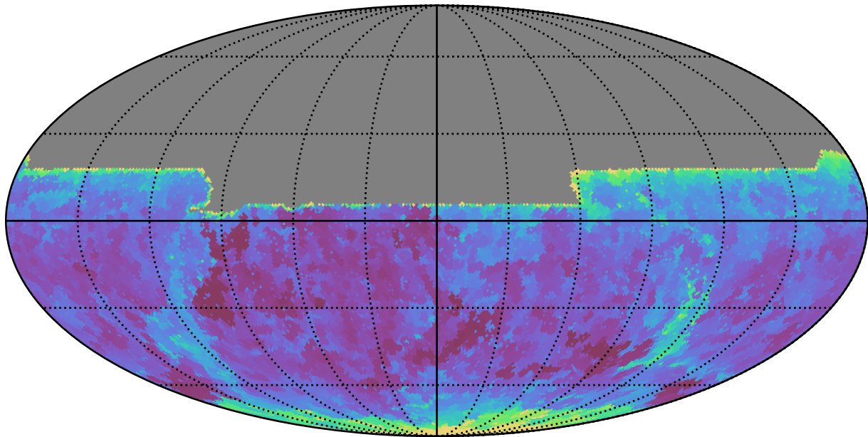
roll_pause_mjdp0_v3.4_10yrs All sky y band: Min seeingEff
