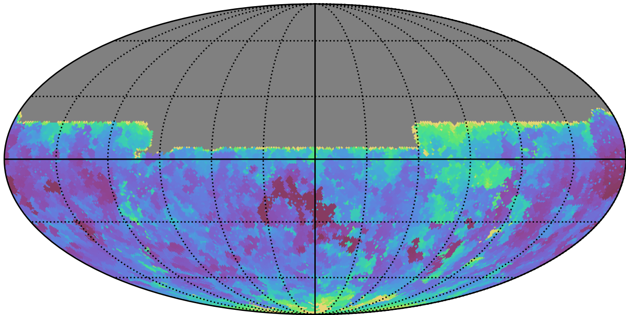
roll_pause_mjdp0_v3.4_10yrs All sky u band: Min seeingEff
