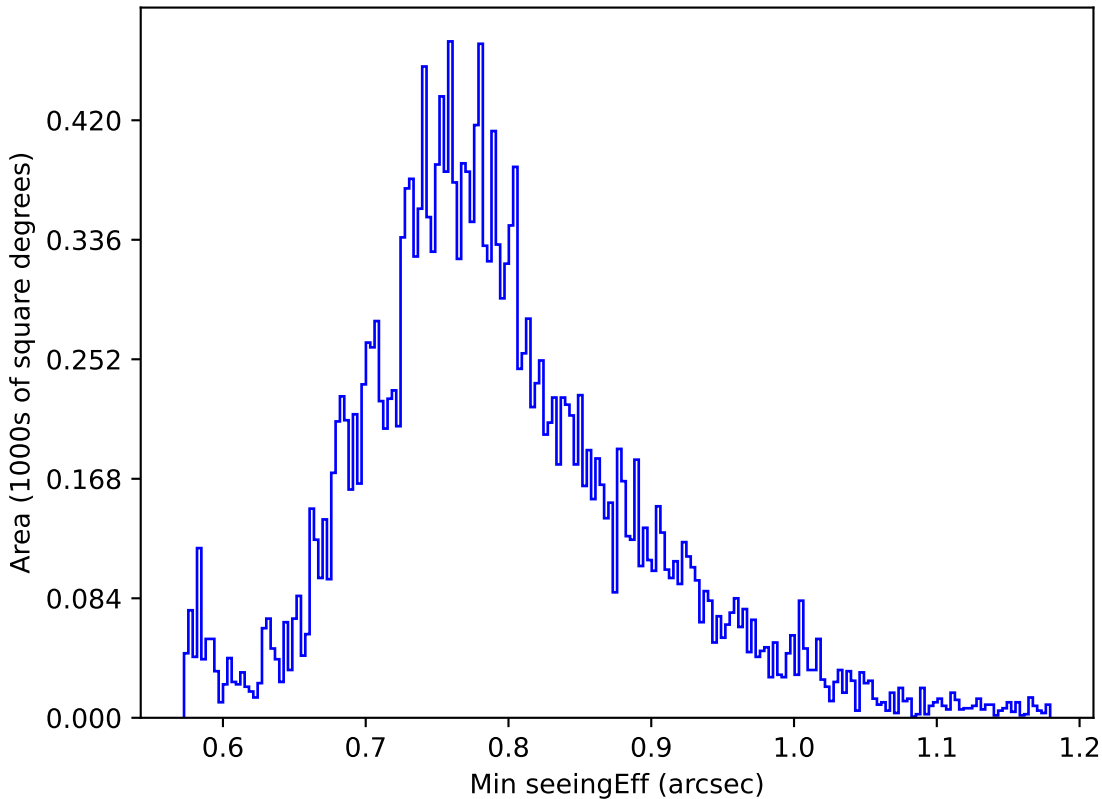
roll_pause_mjdp0_v3.4_10yrs All sky u band: Min seeingEff
