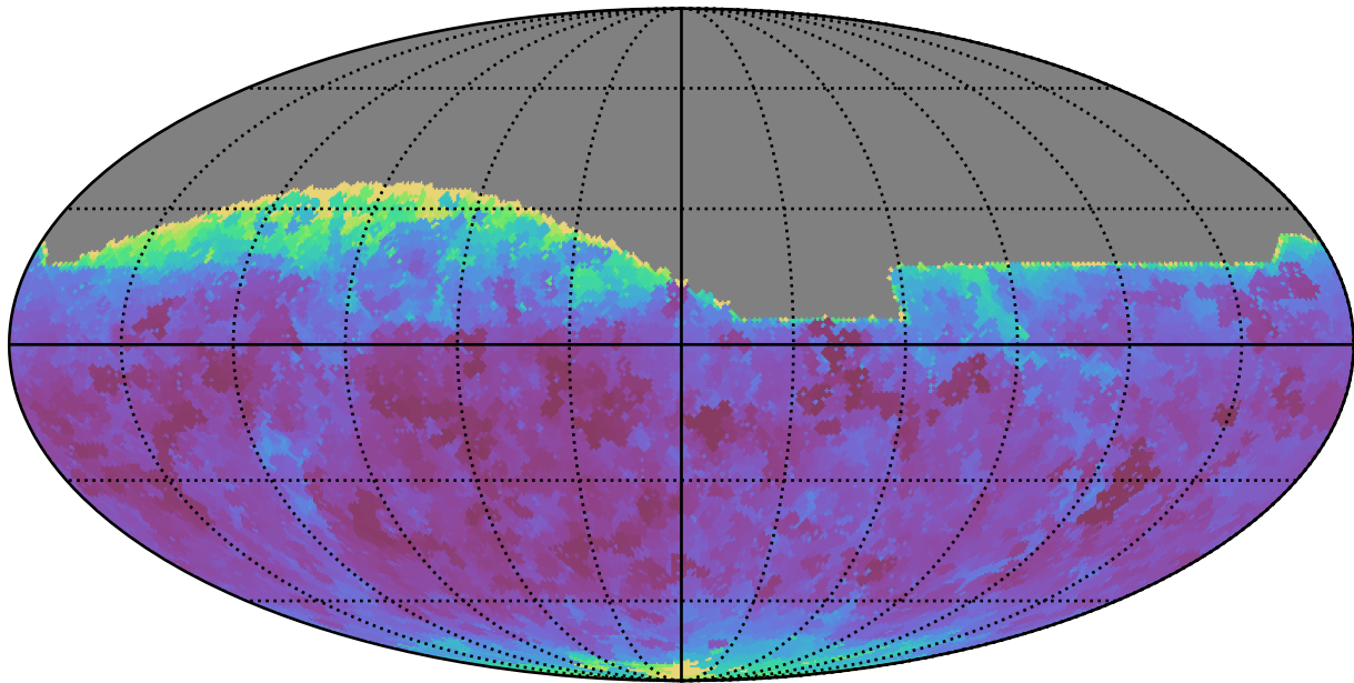
roll_pause_mjdp0_v3.4_10yrs All sky i band: Min seeingEff
