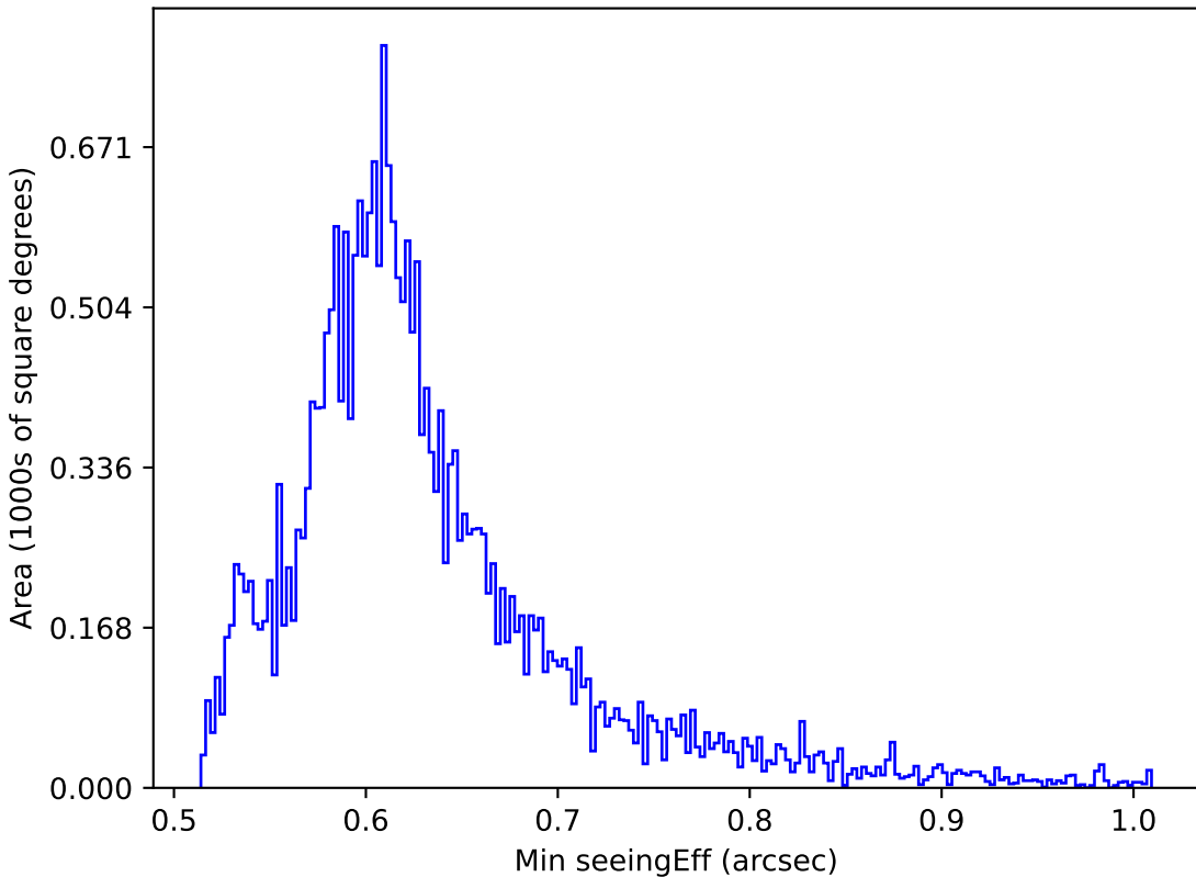
roll_pause_mjdp0_v3.4_10yrs All sky i band: Min seeingEff
