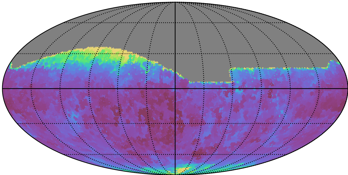
roll_pause_mjdp0_v3.4_10yrs All sky g band: Min seeingEff
