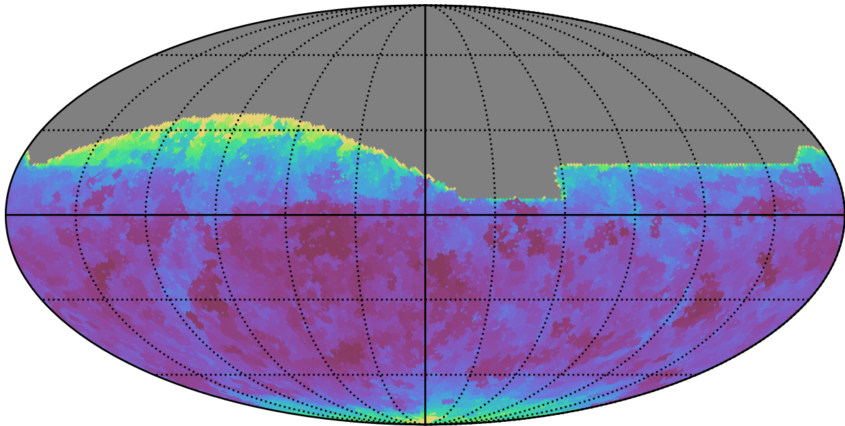
roll_pause_mjdp0_v3.4_10yrs All sky all bands: Min seeingEff
