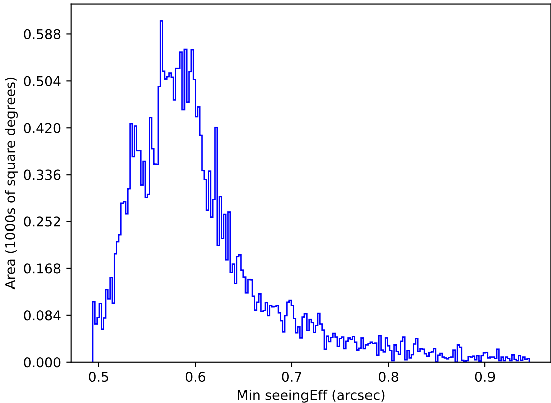
roll_pause_mjdp0_v3.4_10yrs All sky all bands: Min seeingEff
