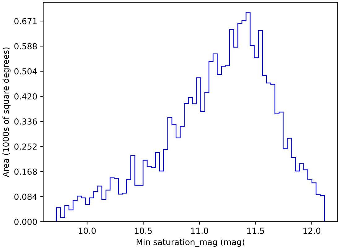
roll_pause_mjdp0_v3.4_10yrs WFD y band: Min saturation_mag
