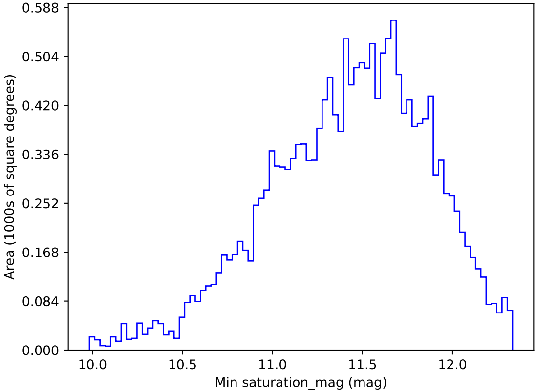
roll_pause_mjdp0_v3.4_10yrs WFD u band: Min saturation_mag
