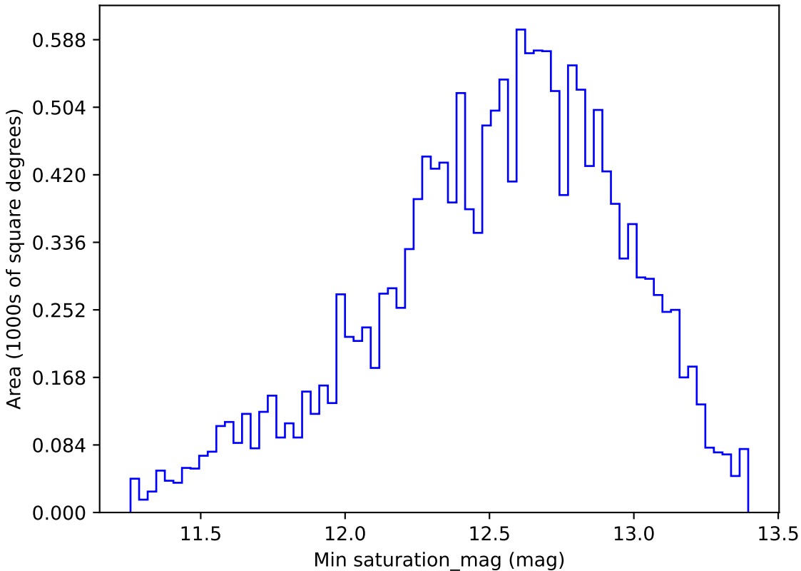
roll_pause_mjdp0_v3.4_10yrs WFD r band: Min saturation_mag
