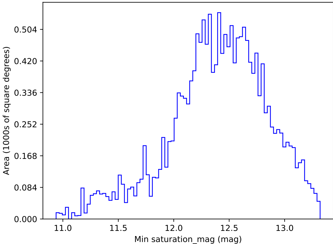
roll_pause_mjdp0_v3.4_10yrs WFD i band: Min saturation_mag
