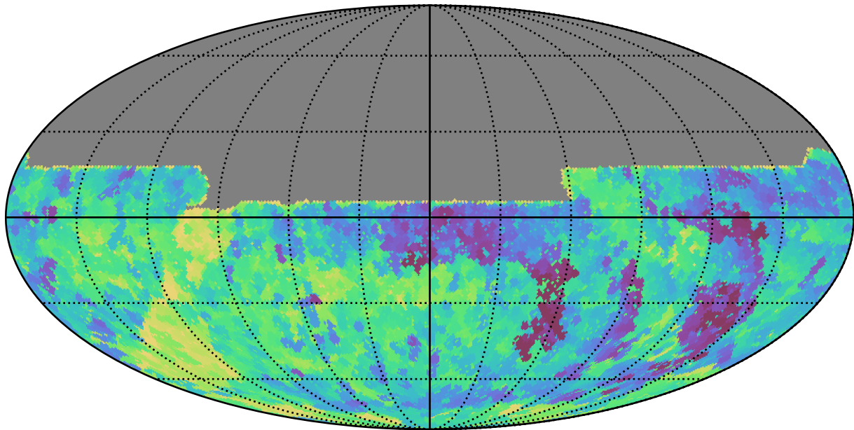
roll_pause_mjdp0_v3.4_10yrs All sky y band: Min saturation_mag
