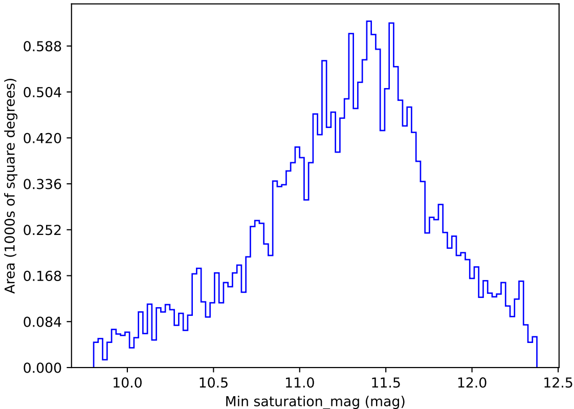
roll_pause_mjdp0_v3.4_10yrs All sky y band: Min saturation_mag
