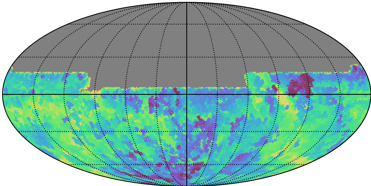
roll_pause_mjdp0_v3.4_10yrs All sky u band: Min saturation_mag
