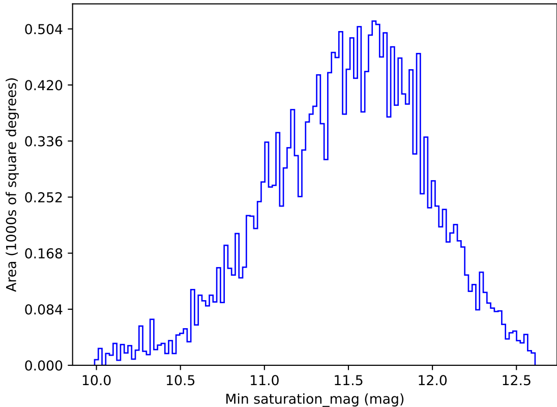
roll_pause_mjdp0_v3.4_10yrs All sky u band: Min saturation_mag
