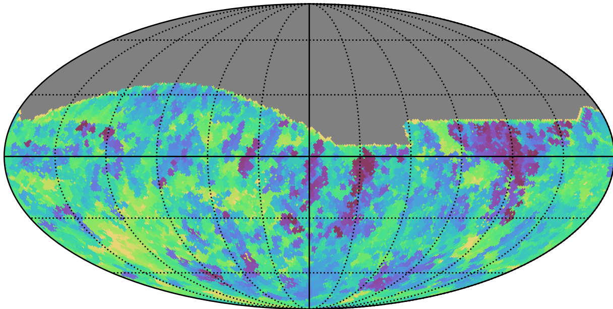
roll_pause_mjdp0_v3.4_10yrs All sky r band: Min saturation_mag
