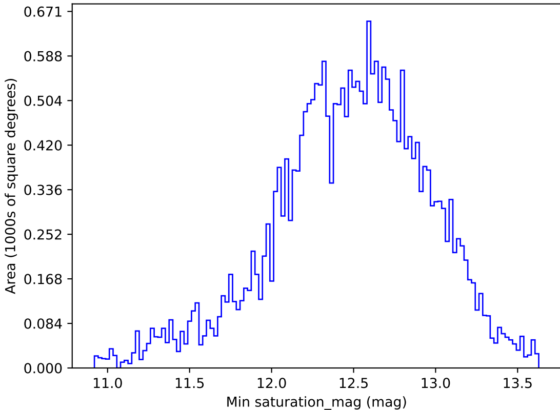
roll_pause_mjdp0_v3.4_10yrs All sky i band: Min saturation_mag
