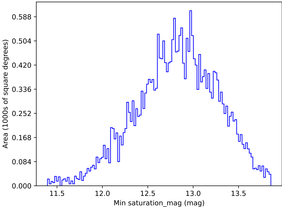
roll_pause_mjdp0_v3.4_10yrs All sky g band: Min saturation_mag
