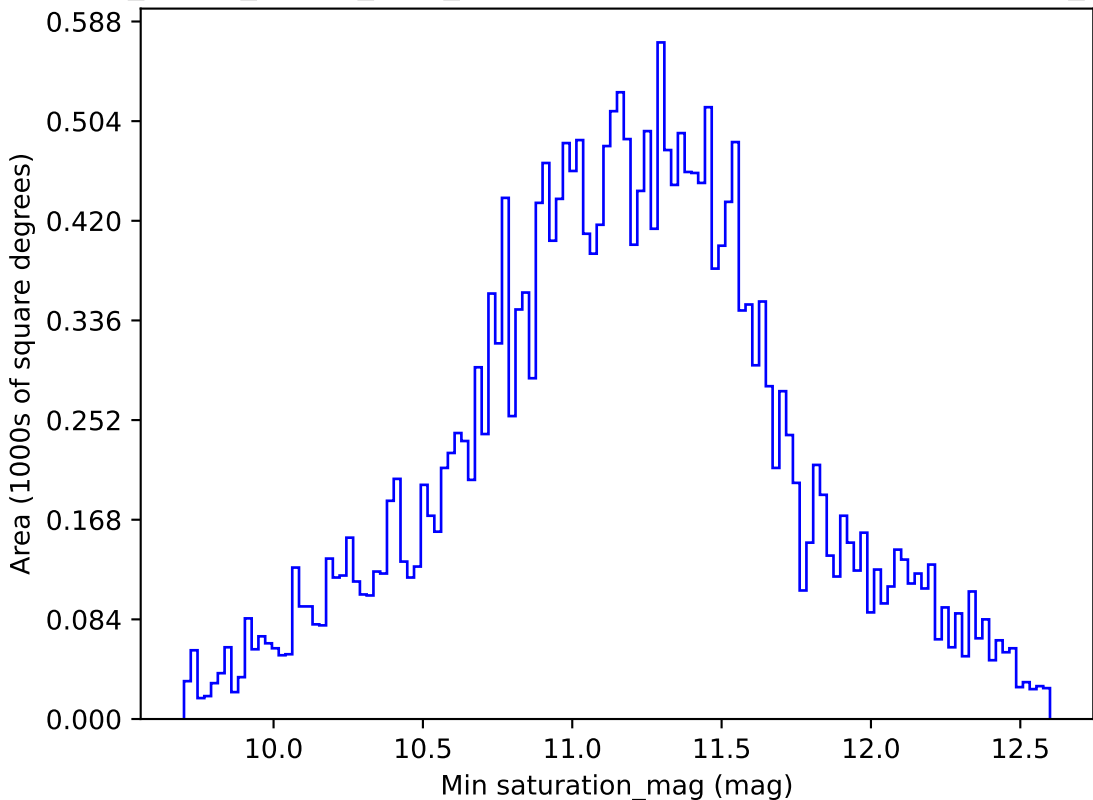
roll_pause_mjdp0_v3.4_10yrs All sky all bands: Min saturation_mag
