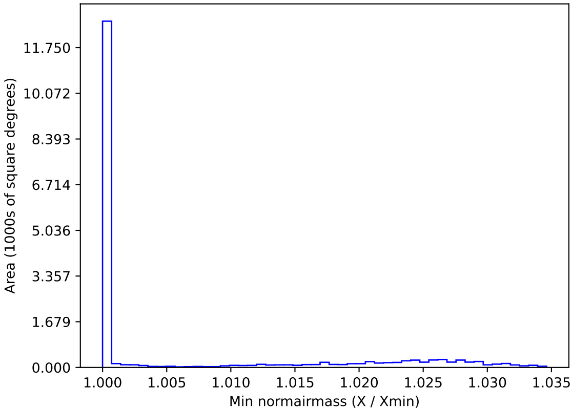
roll_pause_mjdp0_v3.4_10yrs WFD z band: Min normairmass
