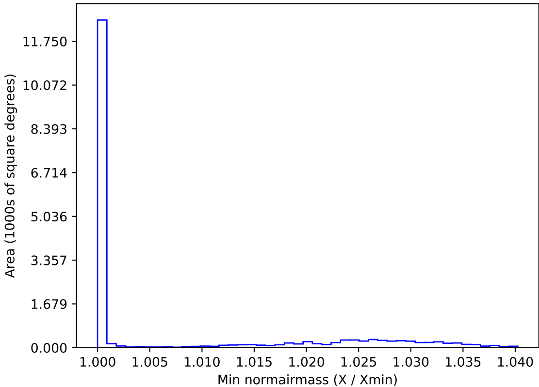
roll_pause_mjdp0_v3.4_10yrs WFD y band: Min normairmass
