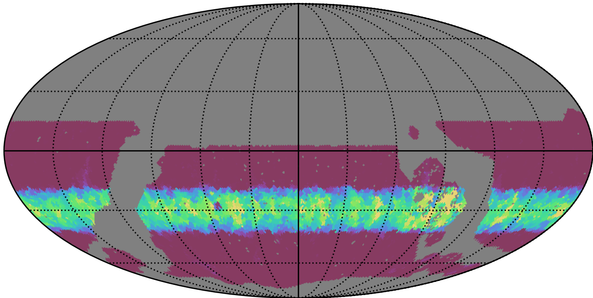
roll_pause_mjdp0_v3.4_10yrs WFD u band: Min normairmass
