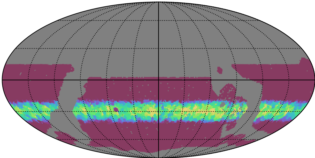
roll_pause_mjdp0_v3.4_10yrs WFD r band: Min normairmass
